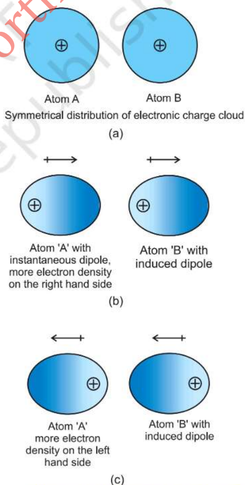
Fig. 5.1 Dispersion forces or London forces between atoms.
