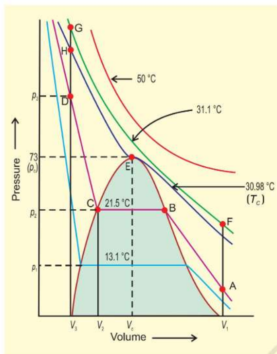
Fig. 5.13 Isotherms of carbon dioxide at various temperatures
